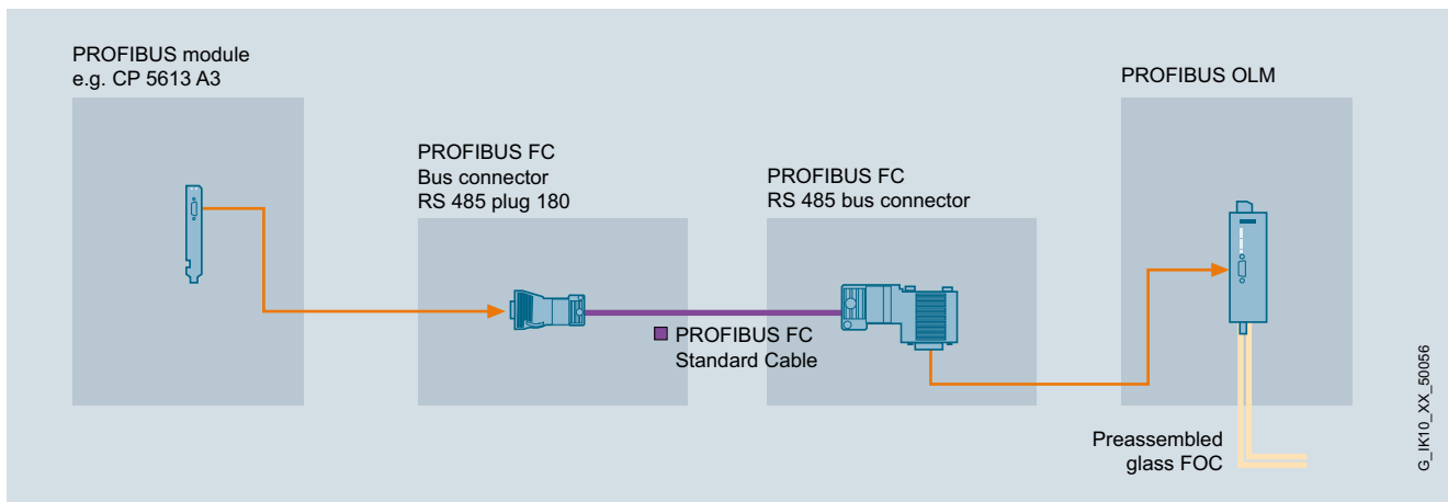
Connection example of optical networking
